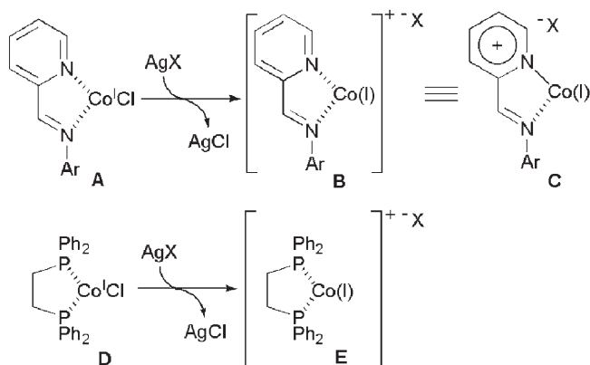
Scheme 2. Postulated intermediate.
