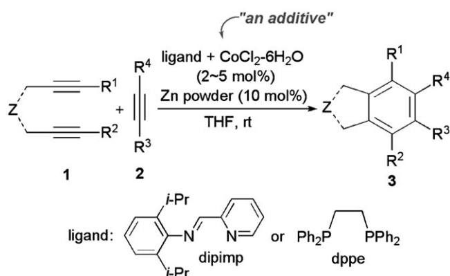
Scheme 1. Ligand/CoCl 2 ·6H 2 O/Zn-catalyzed reaction of alkynes to benzene derivatives.
